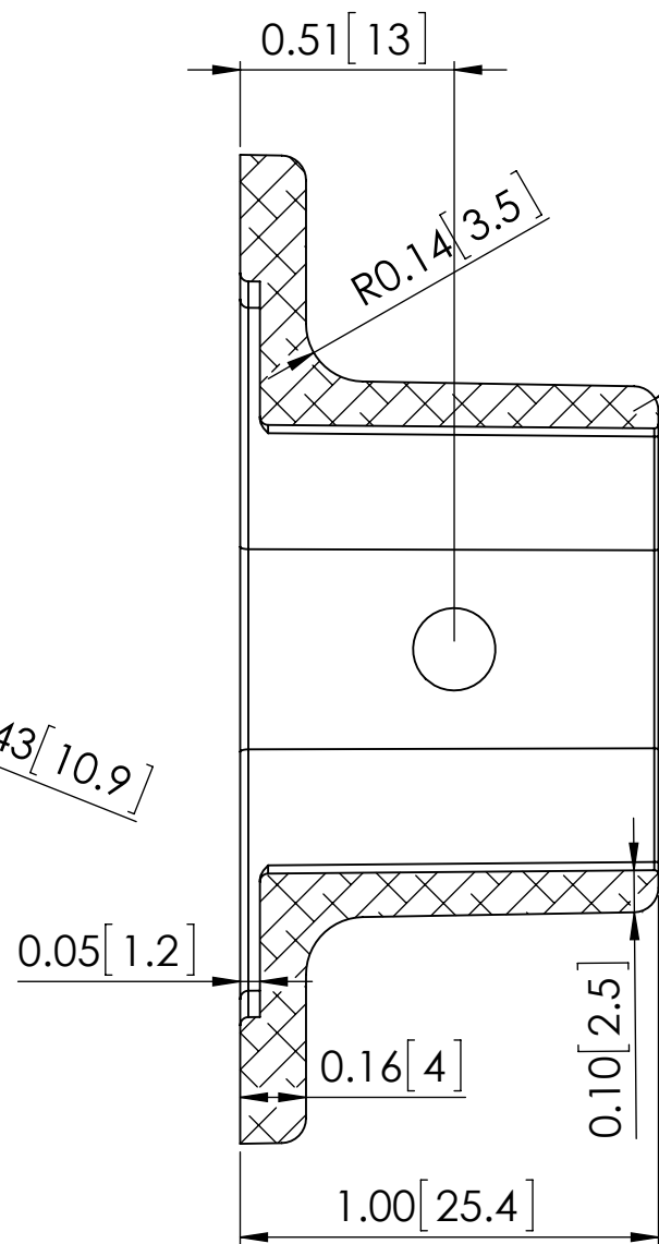
SECTION C-C SCALE 2 : 1
